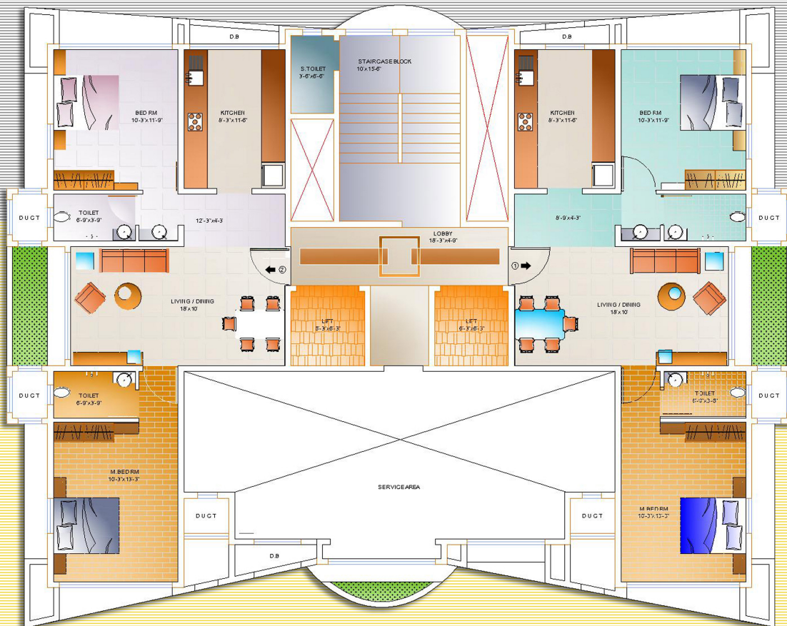
PLAN AT 8TH & 15TH FLOOR
